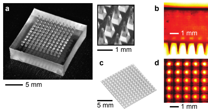
Fig. 2. (a) Photographs of a fabricated prototype PLA microneedle array. (b) An optical side-view transmission image of the microneedle array. Needle length: 1.6 mm, base diameter: 500 \mu m, interspacing: 1 mm, number of needles: 11 by 11, and substrate size: 15 mm by 15 mm \times 4 mm. (c) Photograph of a microlens array. Focal length of lens: 9.5 mm, and substrate size: 15 mm by 15 mm by 2 mm. (d) Optical transmission image of the microlens array.
