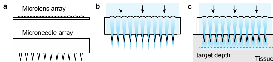
Fig. 1. Design principle of the OMNA. (a) Schematics of a microneedle array and microlens array. (b) Illustration of an assembled OMNA. The microlens array focuses incident light through the microneedles. (c) Illustration of light delivery into a tissue. The design has been optimized to achieve uniform and maximal light intensity at a target depth.
